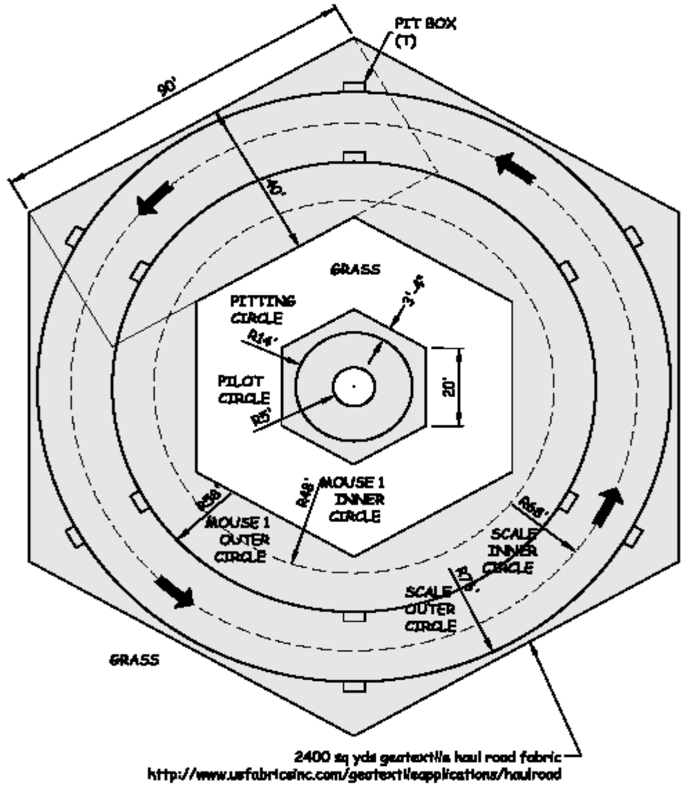
CONTROL LINE FIELD LAYOUT FOR SCALE & MOUSE 1 RACING, & STUNT FLYING
